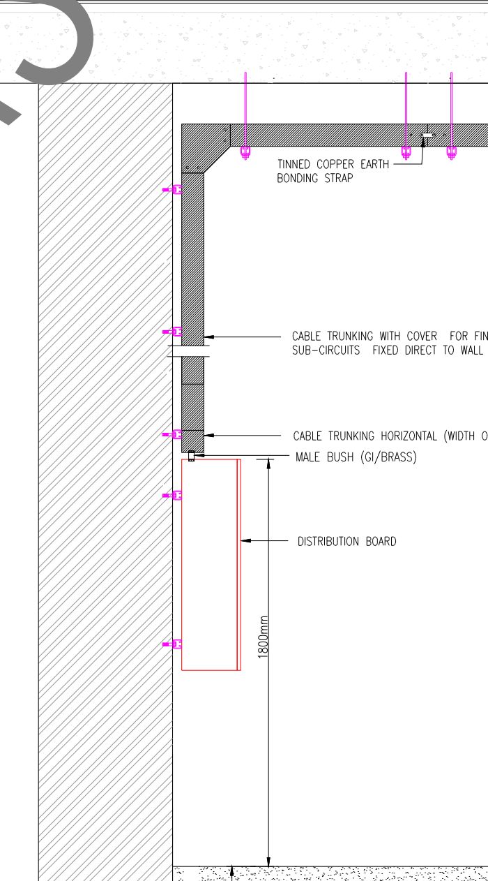
06 SURFACE MOUNTED DISTRIBUTION BOARD NTS
