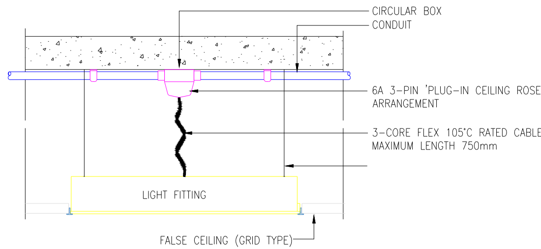
02 TYPICAL INSTALLATION DETAIL FOR RECESSED LED LUMINAIRE SCALE NTS
