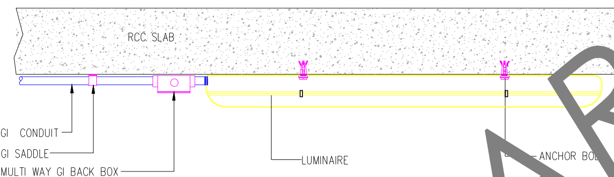
05 TYPICAL INSTALLATION DETAIL FOR SURFACE LED LUMINAIRE SCALE NTS
