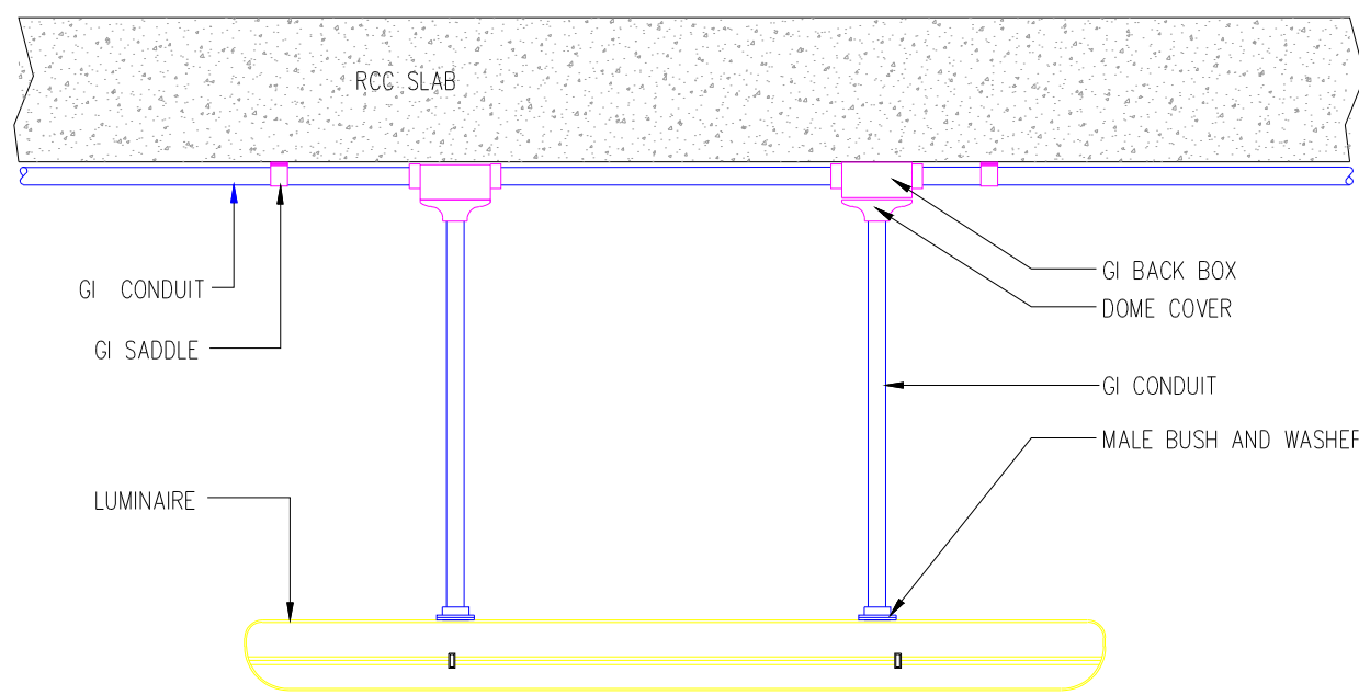
01 TYPICAL INSTALLATION DETAIL FOR SUSPENDED LED LUMINAIRE SCALE NTS
