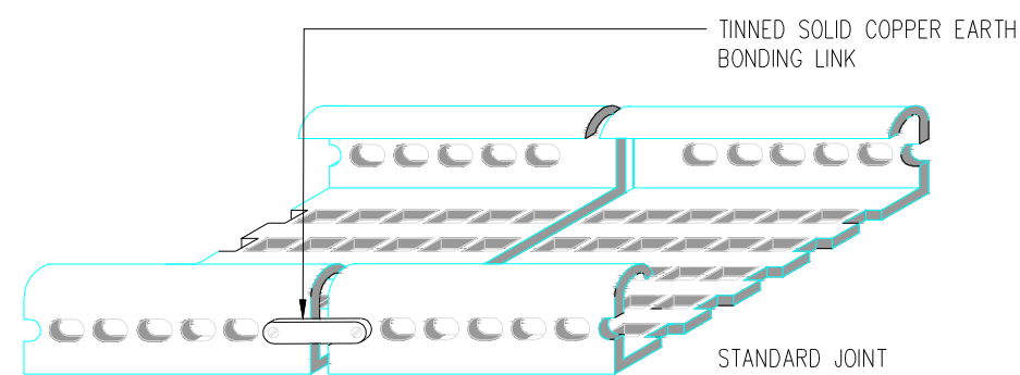
04 CABLE TRAY BONDING NTS
