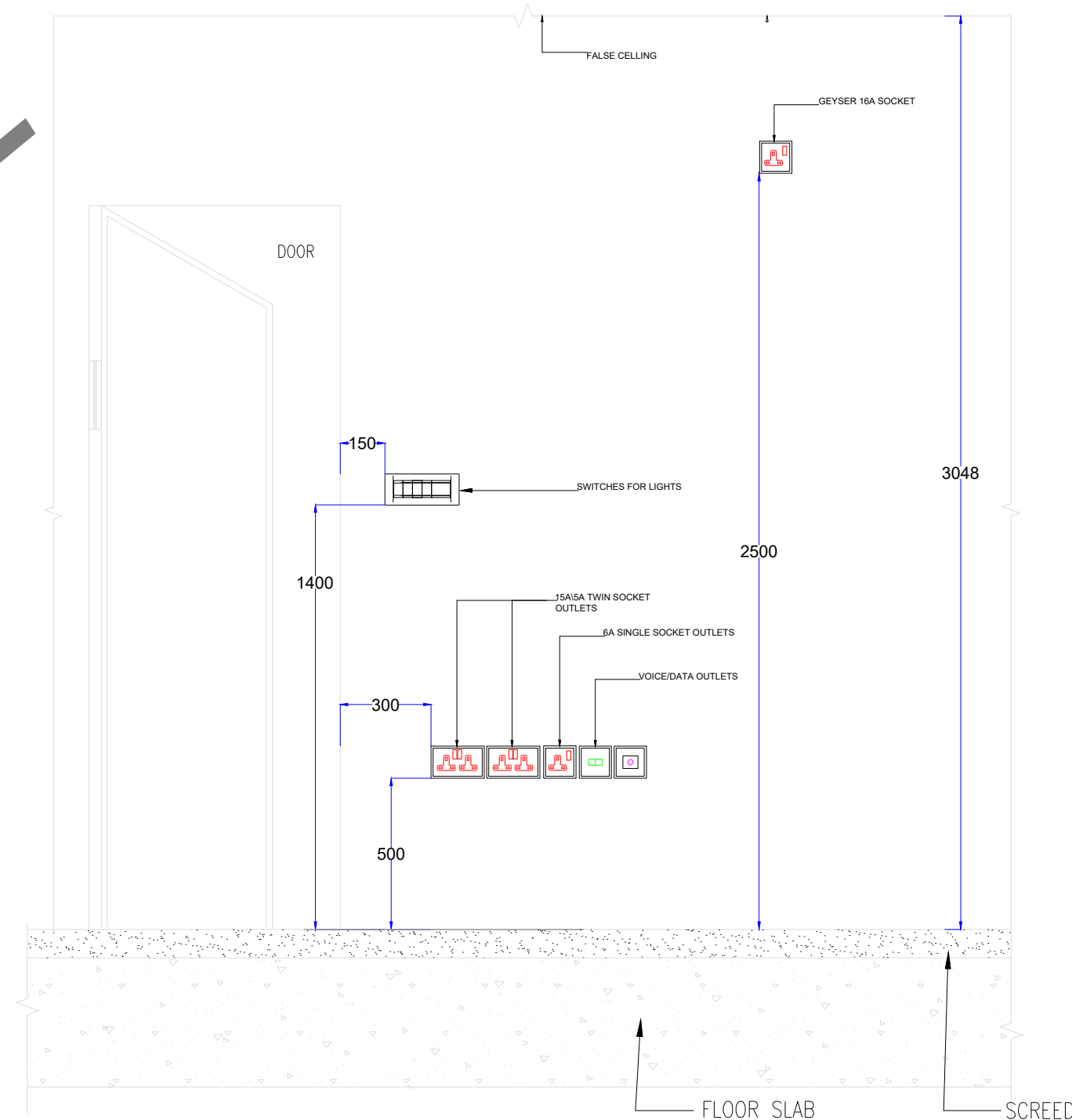
08 SWITCHBOARDS NTS
