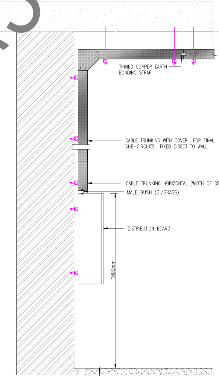
06 SURFACE MOUNTED DISTRIBUTION BOARD NTS
